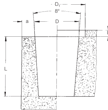
Mounting hole®
