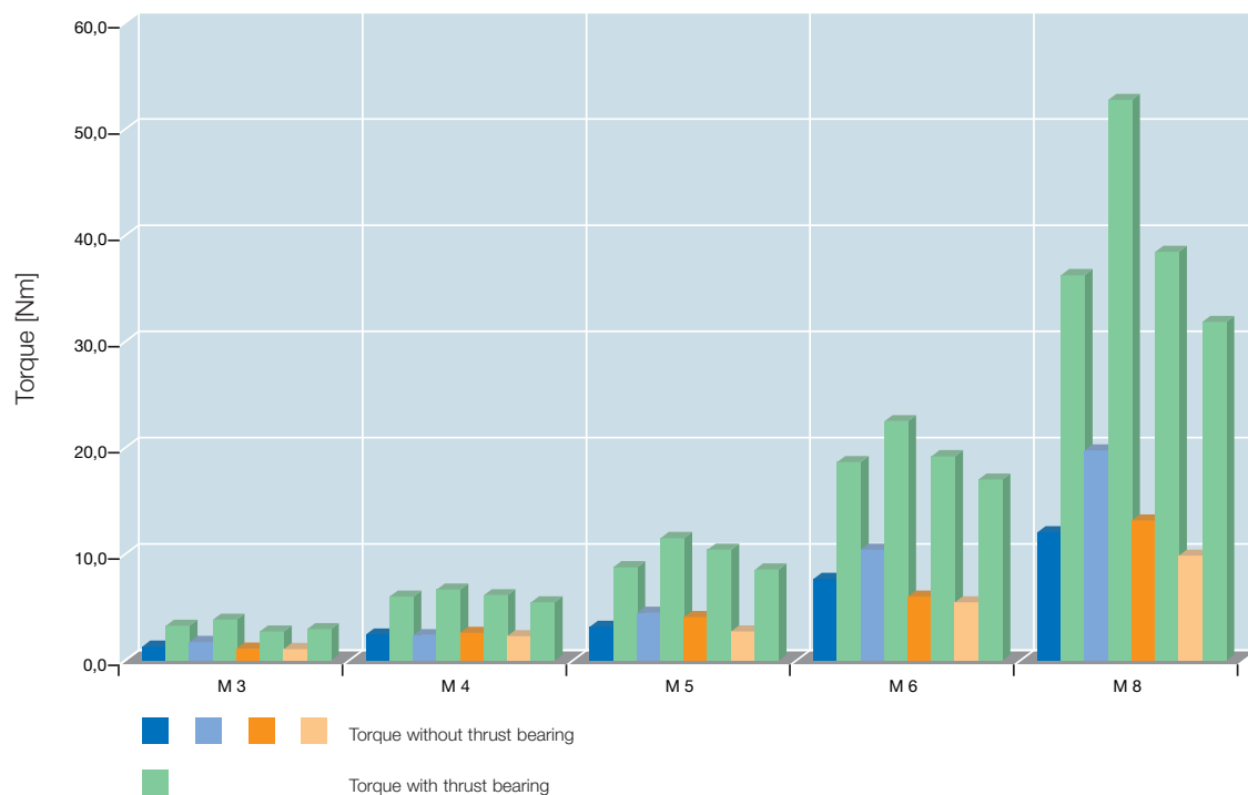
Torque values QUICKSERT® M 3 to M 8
